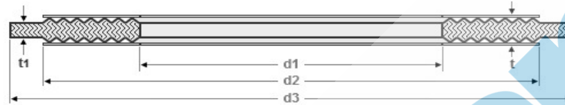
Dimensions of Grooved Metal Gaskets as Per ASME B16.20 to Suit ASME B16.47 Series A Flange
