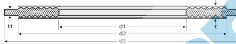
Dimensions of Grooved Metal Gaskets as Per ASME B16.20 to Suit ASME B16.47 Series B Flange
