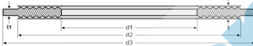
Dimensions of Grooved Metal Gaskets as Per ASME B16.20 to Suit ASME B16.5 Flange
