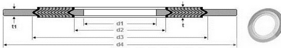
Dimensions of Spiral Wound Gaskets as per ASME B16.20 to suit ASME B16.5 Flange
