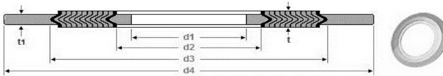
Dimensions of Spiral Wound Gaskets to suit for MSS SP44 Flange.
